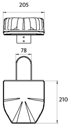
AURA NOCTILED TOP 60 mm
