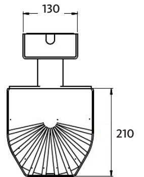
AURA NOCTILED APPLIQUE
